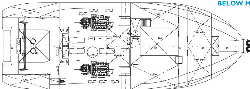
BELOW MAINDECK
